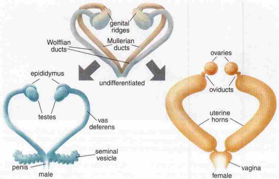
Figure 3. Mouse reproductive anatomy begins to develop ten or 11 days after conception. As shown in this schematic drawing, the precursors of both the male and female internal organs (Wolffian and Mullerian duct systems respectively) are present at first. In males, the undifferentiated genital ridges develop into testes around day 12 and produce hormones that cause the regression of the Mullerian ducts and the differentiation of the Wolffian ducts into the vas deferens and seminal vesicles. In females, the ovaries differentiate slightly later in development. In the absence of male hormones, the Mullerian ducts develop into the uterus and oviducts.
